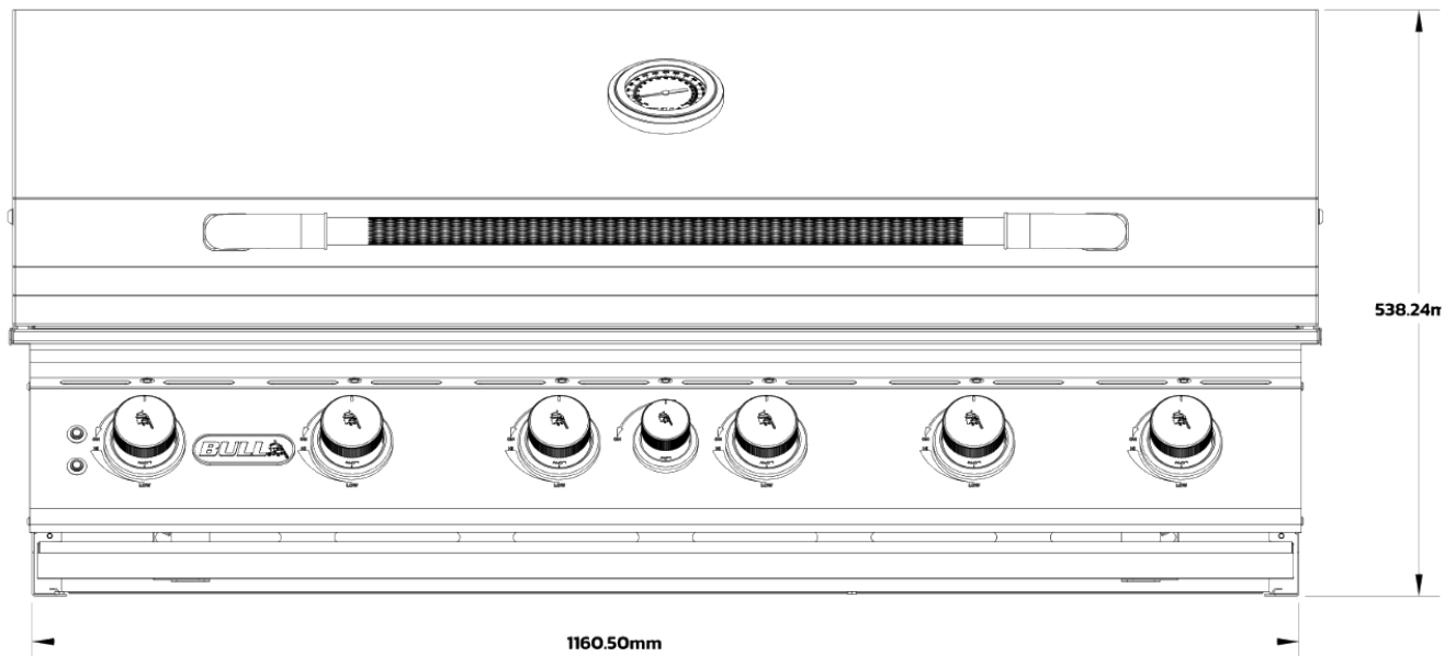
FRONT VIEW 1160.50 W × 538.24 H mm
