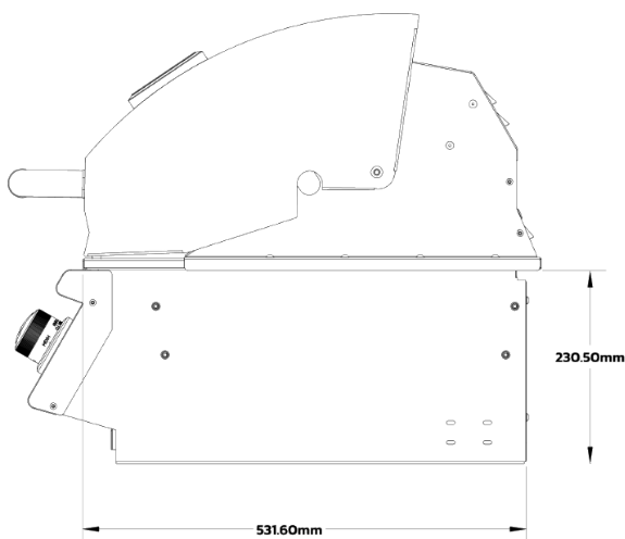
SIDE VIEW 531.60 D × 230.50 H mm
